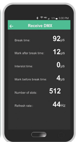
DMX Tester
