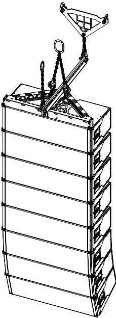
GSL8/12 Line array 8-deep Tension mode - Front
