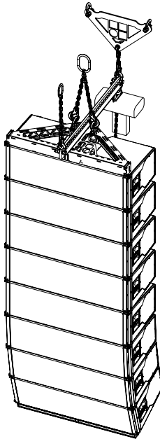
GSL8/12 Line array 8-deep Compression mode with motor - Front
