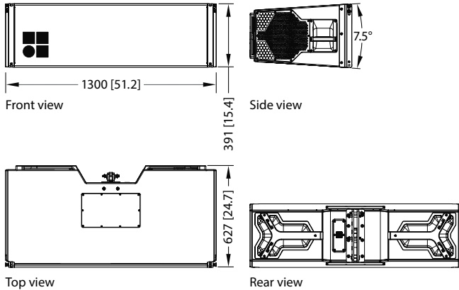
GSL12 cabinet dimensions in mm [inch]
