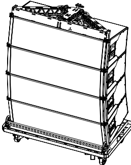
E7490 4 x GSL8/GSL12 Touring cart Loaded in Tension mode with mounted GSL Flying frame
