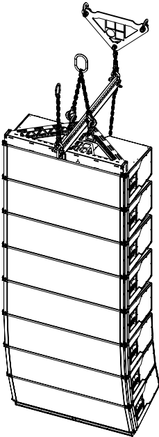
GSL8/12 Line array 8-deep Compression mode - Front
