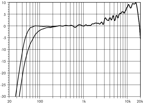
GSL12 frequency response, standard and CUT modes* * single cabinet within array
