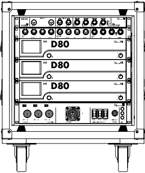
Z5570/Z5571 3x D80 Touring rack OUT: 1x LKA 25/3 x NL8
