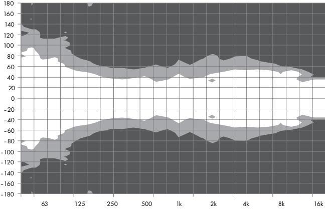
GSL12 horizontal dispersion characteristics 2
